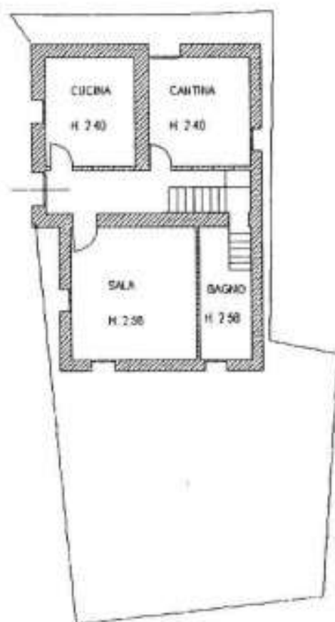
PIANO TERRA
